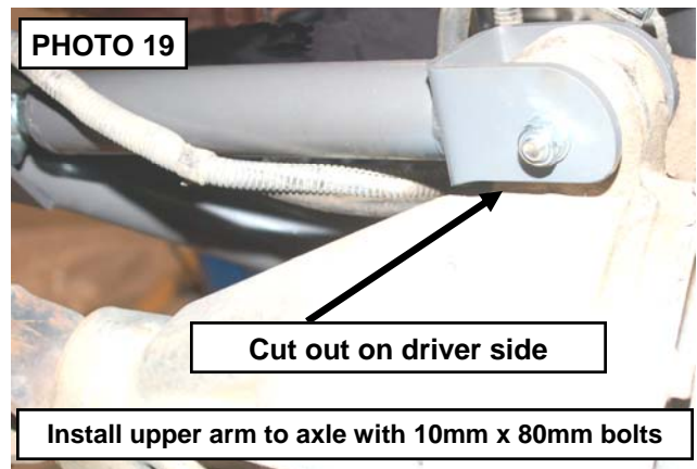
Install the upper arm to lower using 10MM X 80MM bolts
