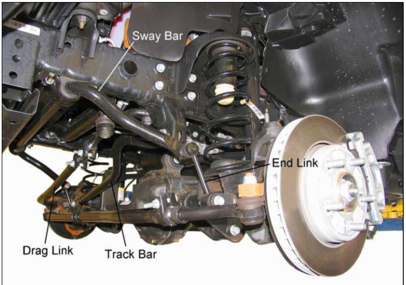
Front Suspension
