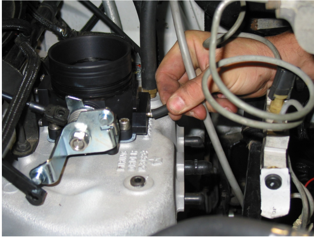
Figure 4.4 PERFECT MAP sensor vacuum hose connection
