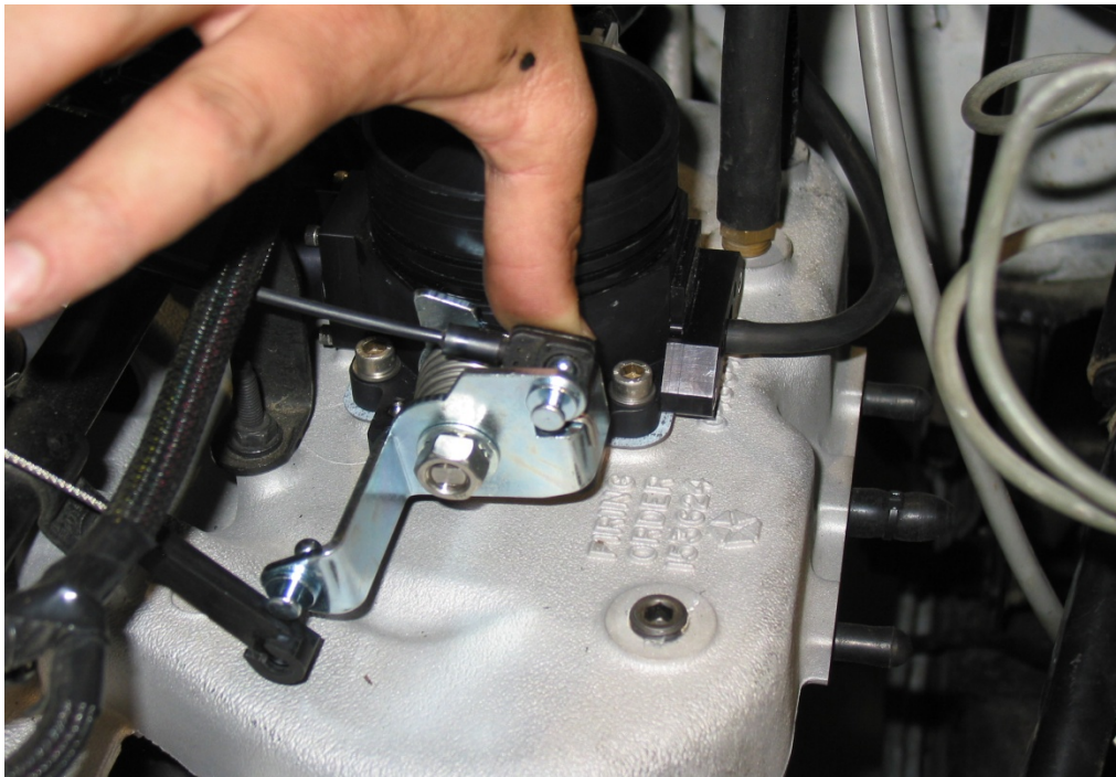
Figure 4.1 Throttle and Kickdown Cables
